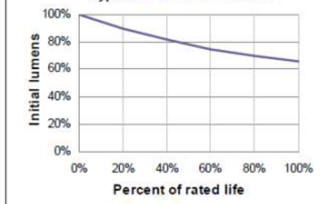
Typical lumen maintenance
